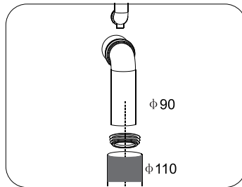
2.2.3 Use the pipe gasket to connect the waste pipe of \phi 90 mm and \phi 110 mm.
