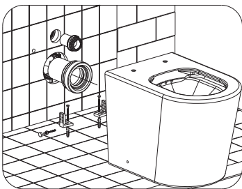
2.4.7 Measure the distance for the anchor screws and fix them on the floor. Apply the sealant to both pipes, then insert them into the cistern and install the toilet.
